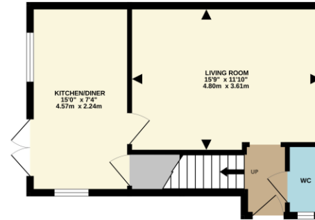
GROUND FLOOR 367 sq.ft. (34.1 sq.m.) approx.
