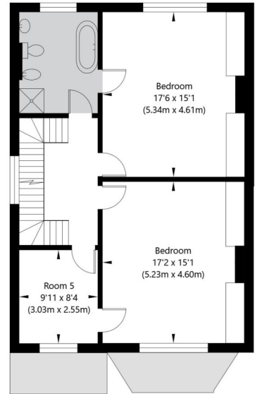
First Floor GROSS INTERNAL FLOOR AREA APPROX. 78.33 SQ M / 843 SQ FT
