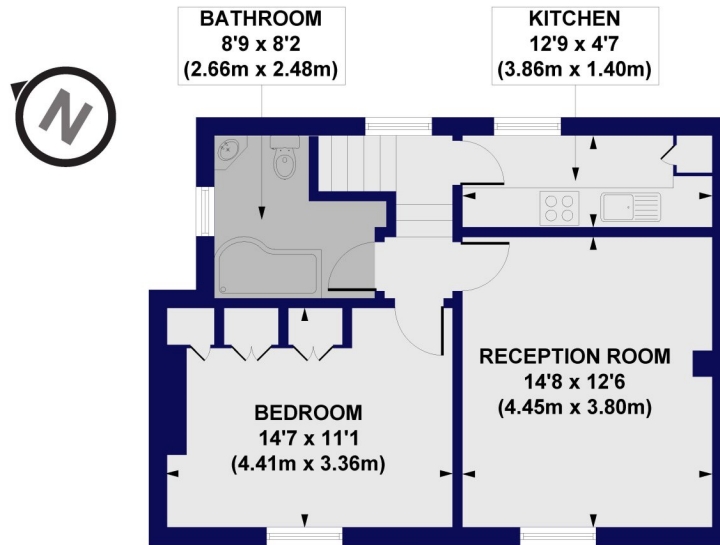
SECOND FLOOR GROSS INTERNAL FLOOR AREA 523 SQ FT
